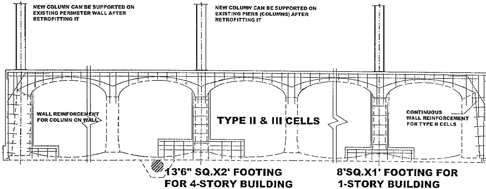
FIG. 6-5: PRESERVE CELLS BUILDING CONSTRUCTION DEVELOPMENT
